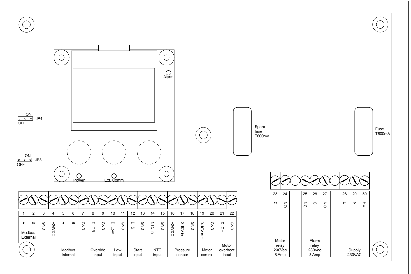
Fig. 2 Connectors overview
