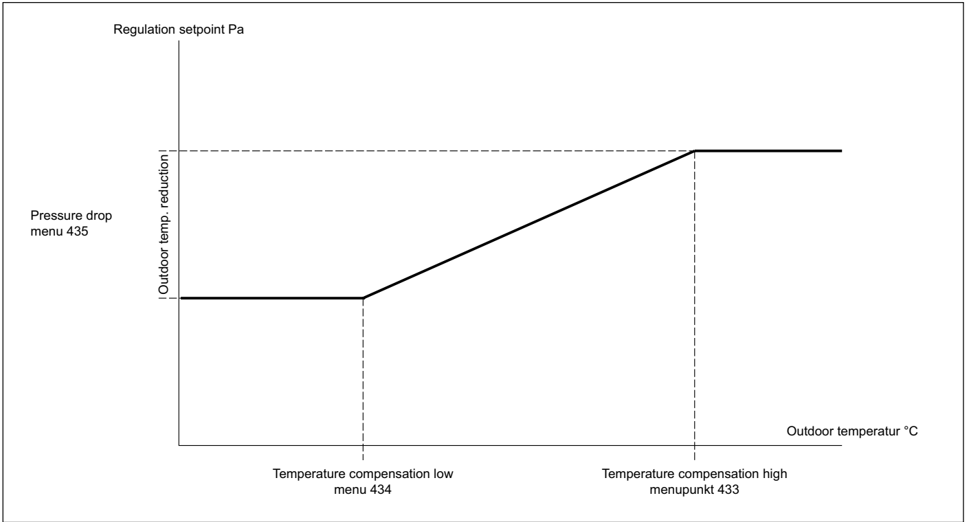
Fig. 4 Temperature compensation
