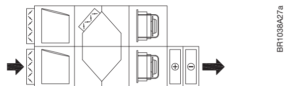
Cross exchanger AHU
