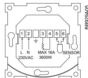
Anschlüsse
